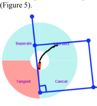
Figure 5. Drawing a circle within a given square
