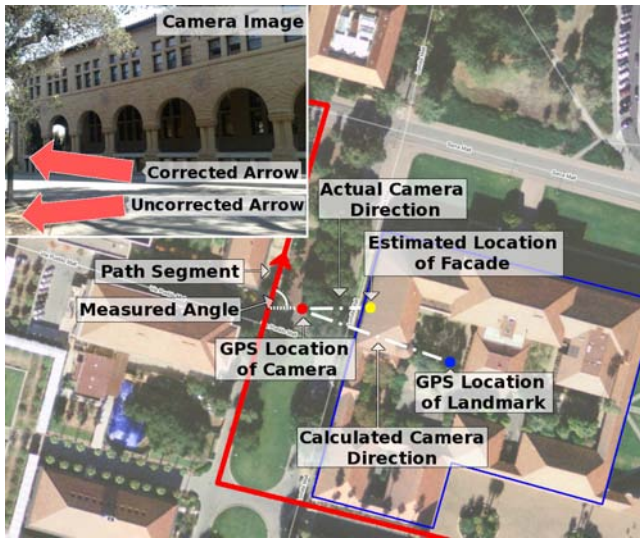
Figure 5. Example of calculating orientation of arrows for image augmentation. The angle between the current path segment and the camera direction defines the arrow placement in the context of the camera image. Compare the result indicating a path parallel to building using the corrected arrow (from the cluster location) to the uncorrected arrow (from the original GPS location) in the inset camera image.
