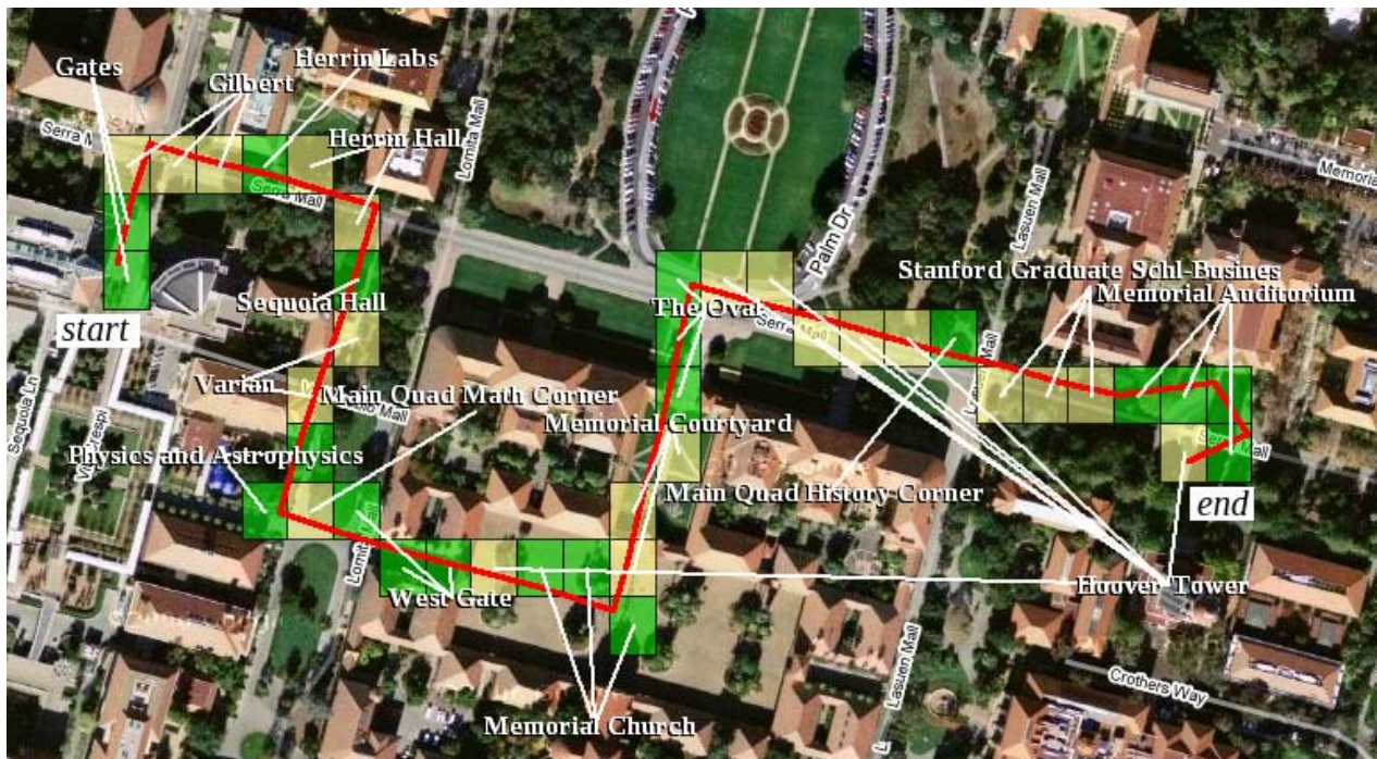
Figure 4. A sample tour path and the loxels that the path intersects. White lines pointing from loxel to a landmark along the path indicate that this landmark is the best for navigation directions for that loxel. The loxel color changes whenever the previous loxel along the path uses a different landmark for navigation directions.
