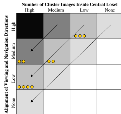
Figure 3. Ordering of clusters based on their alignment with navigation direction and closeness to the navigation path.
