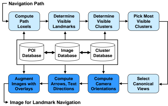
Figure 2. Block diagram for selecting navigation photographs and augmenting them with directions. The first five steps select photographs and the next three steps augment the photographs.
